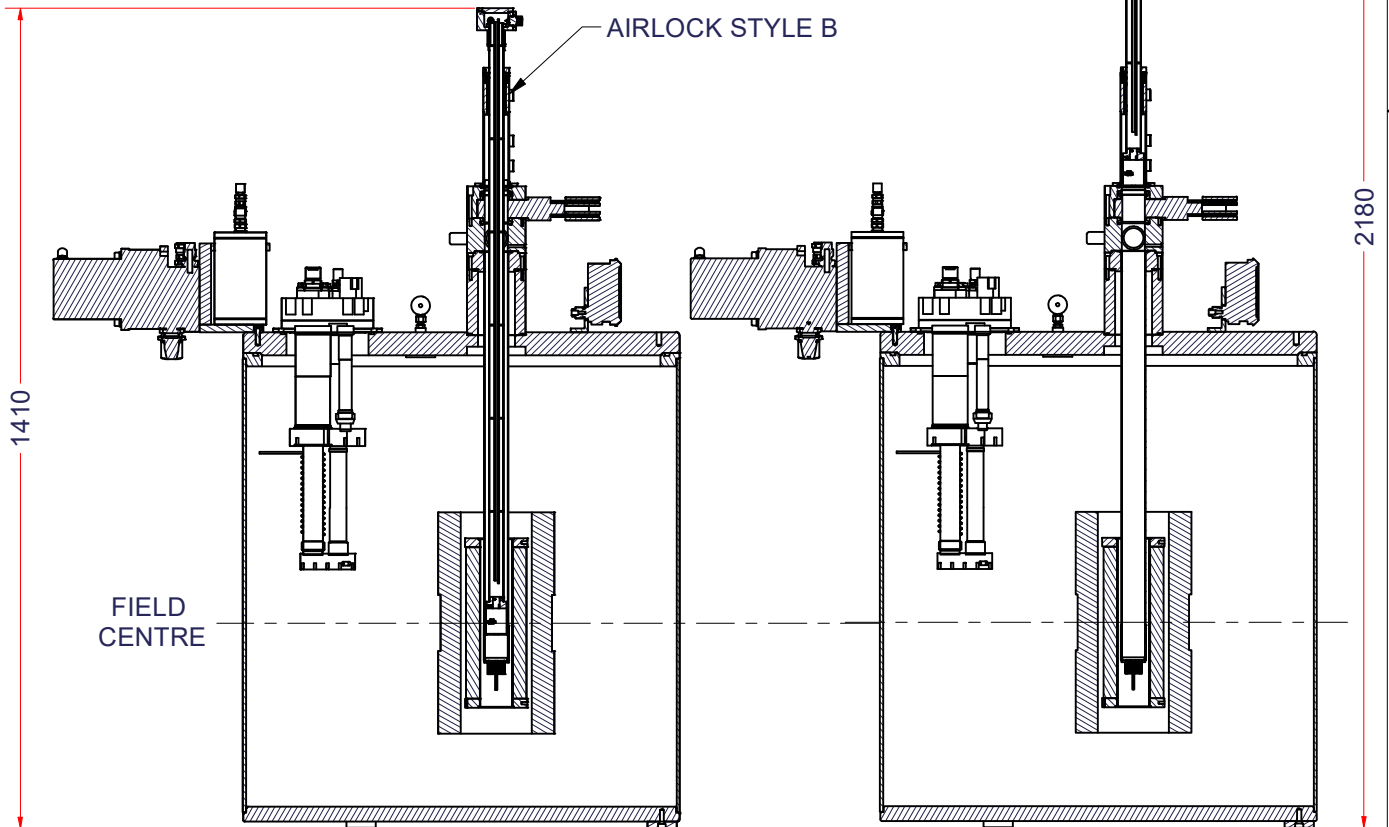
QHR PROBE AT FIELD CENTRE E-E (1 : 13)
